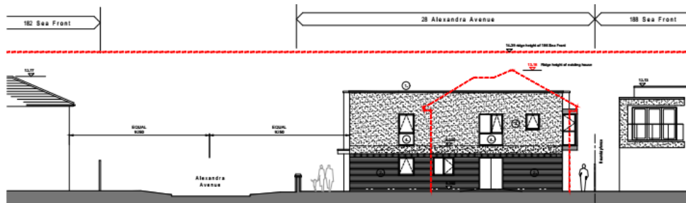
Rear Elevation (North)
