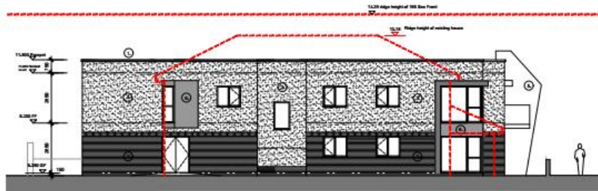
Side Elevation (West)
